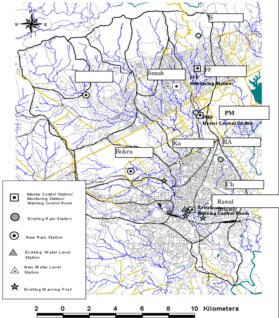
General Layout of Flood Forecasting and Warning System
